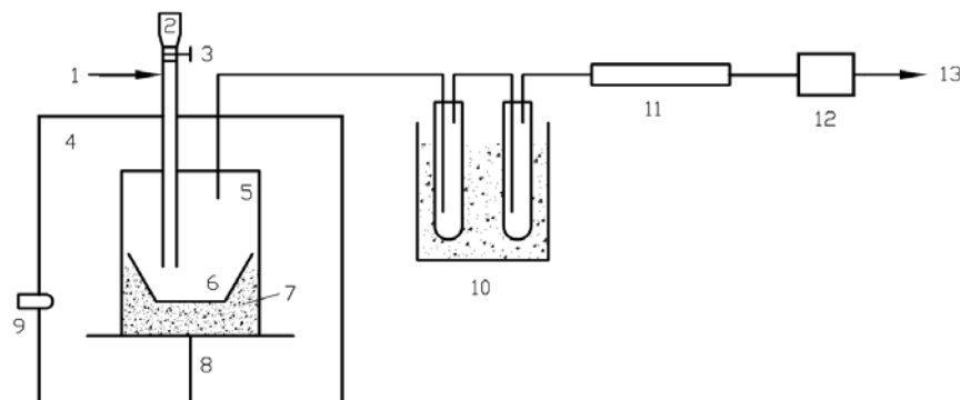
Fig. 1. Schematic diagram of the microwave pyrolysis system
