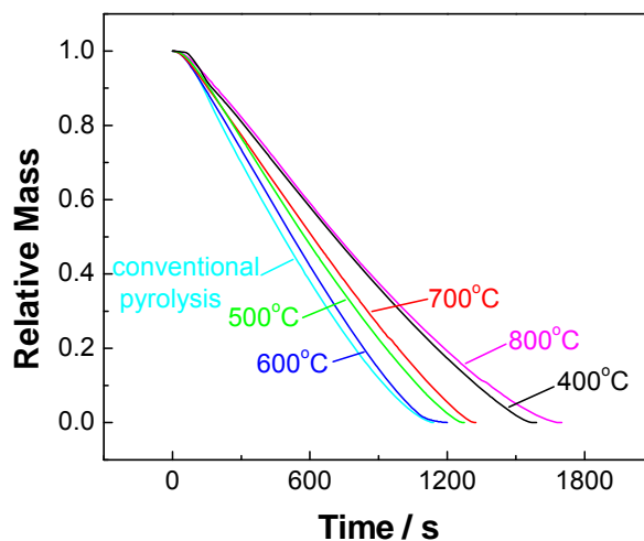
Fig. 6. TG curves for CO 2 gasification of chars under microwave and conventional heating (reactivity test gasification temperature = 1000°C)
