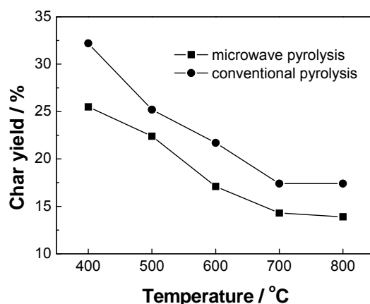
Fig. 2. Variation of the char yields from microwave and conventional pyrolysis with pyrolysis temperature
