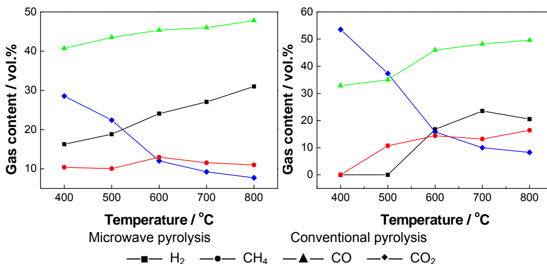
Fig. 3. Main gas components obtained by microwave and conventional pyrolysis at different temperatures
