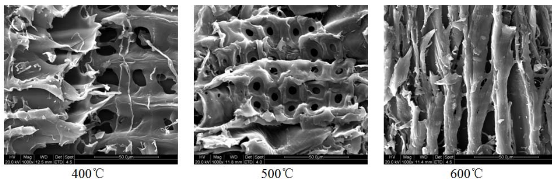
Fig. 5. SEM of char from microwave pyrolysis
