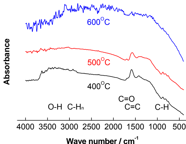
Fig. 4. IR spectra of char from microwave pyrolysis
