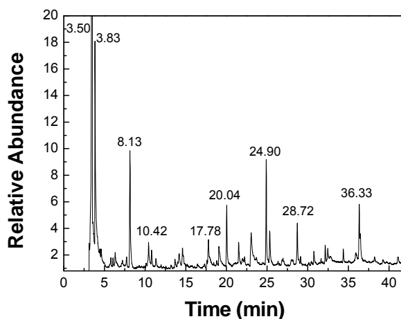
Fig. 7. Total ion chromatogram of tar from pine sawdust microwave pyrolysis at 500°C
