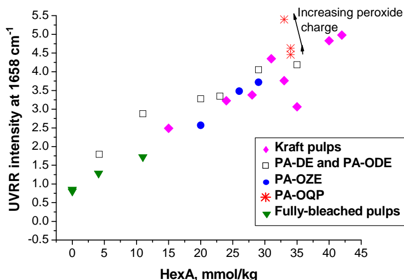
Fig. 16. Correlation of the intensity of the deconvoluted UVRR band at 1658\text{ cm}^{-1} nm with hexenuronic acid group content of the pulps.
