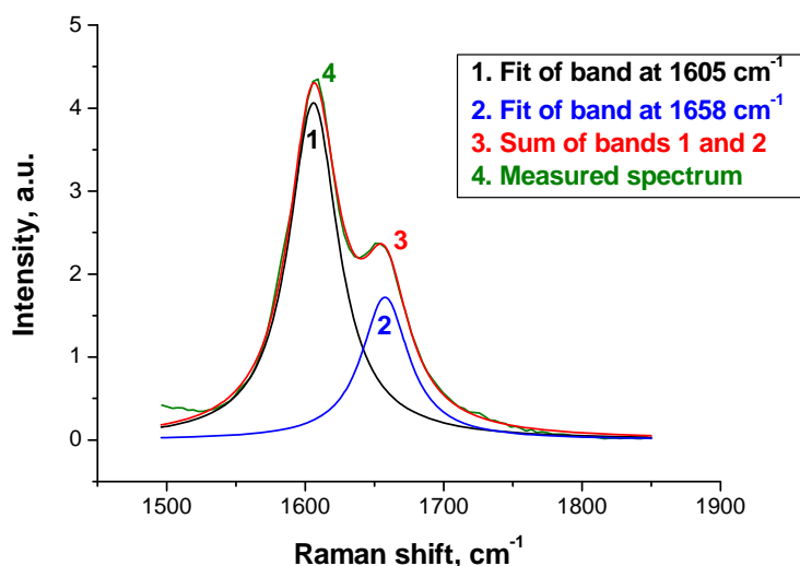
Fig. 1. Least-square fit of Lorentzian curves in the spectral range of 1500-1700 \text{cm}^{-1} for the PA-OEDP sample.
