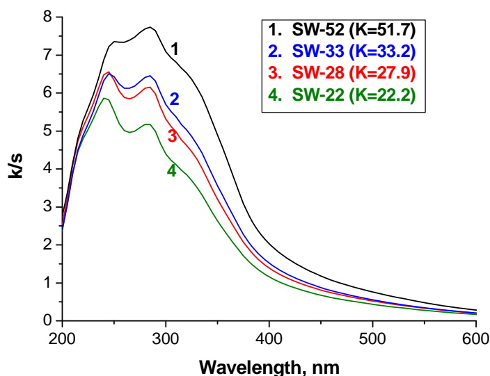
Fig. 3. UV-Vis spectra of unbleached softwood (SW) kraft pulps with kappa numbers 22-52. The reflectance spectra were converted into k/s spectra.
