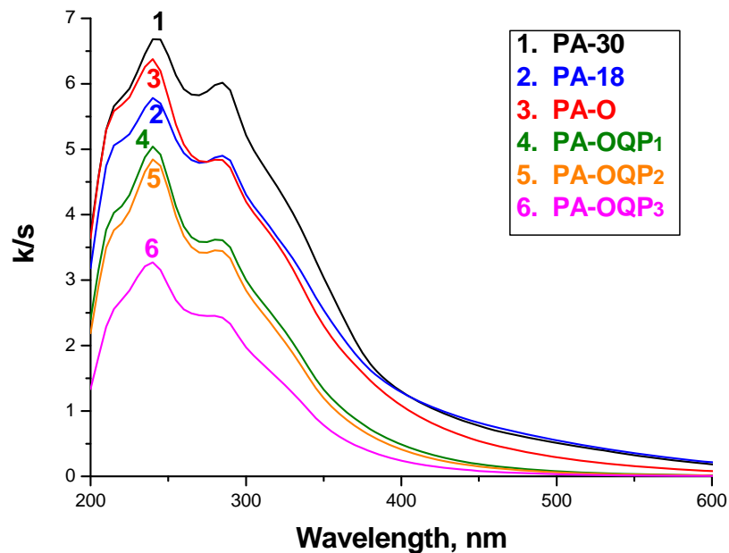
Fig. 9. UV-Vis spectra of profiled alkaline-cooked (PA) pulps bleached with hydrogen peroxide, converted into k/s curves. Peroxide charge increased in order PA-OQP 1 <PA-OQP 2 <PA-OQP 3 .
