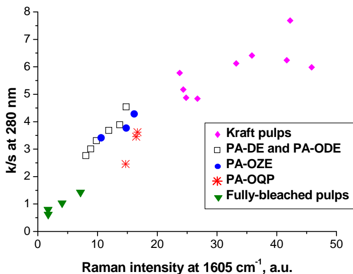
Fig. 14. Correlation of UV-Vis absorption band at 280 nm to Raman band at 1605 cm -1 .
