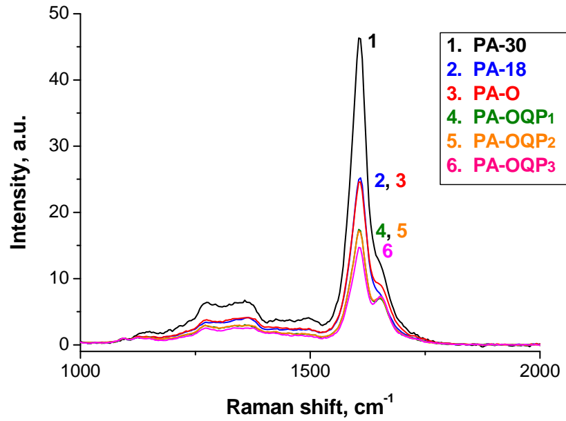
Fig. 8. UVR spectra of profiled alkaline-cooked (PA) pulps bleached with hydrogen peroxide. Peroxide charge increased in order PA-OQP 1 <PA-OQP 2 <PA-OQP 3 .
