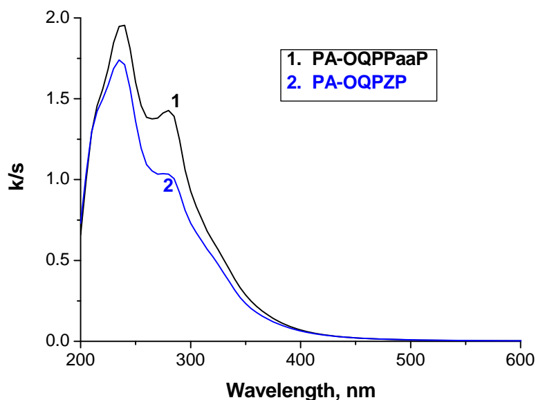
Fig. 11. UV-Vis spectra of PA-OQPPaaP and PA-OQPZP pulps, converted into k/s curves.
