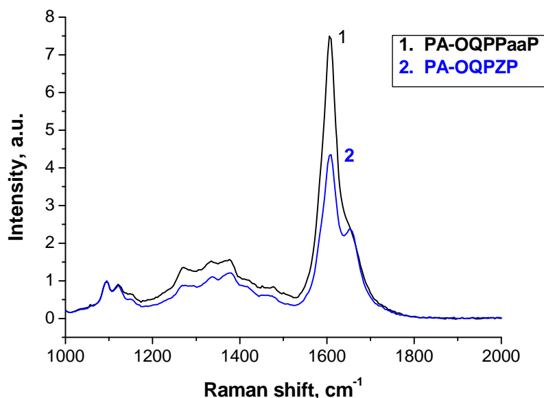
Fig. 10. UVRR spectra of PA-OQPPaaP and PA-OQPZP pulps.
