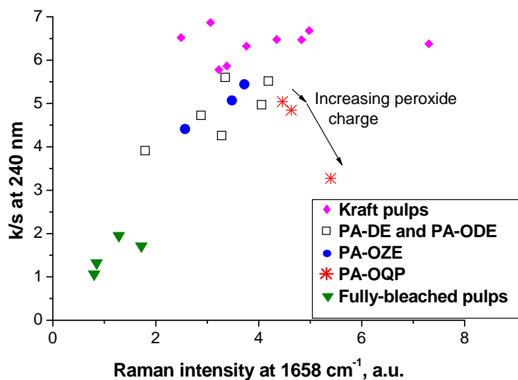
Fig. 15. Correlation of UV-Vis absorption band at 240 nm to Raman band at 1658 cm -1 .
