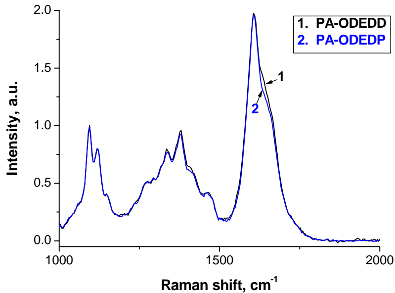
Fig. 12. UVRR spectra of PA-OEDDD and PA-OEDDP pulps.
