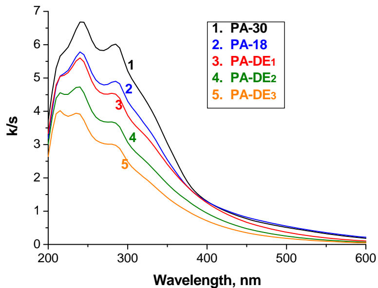
Fig. 7. UV-Vis spectra of profiled alkaline-cooked (PA) pulps bleached with chlorine dioxide, converted into k/s curves. Chlorine dioxide charge increased in order PA-DE_1 < PA-DE_2 < PA-DE_3 .
