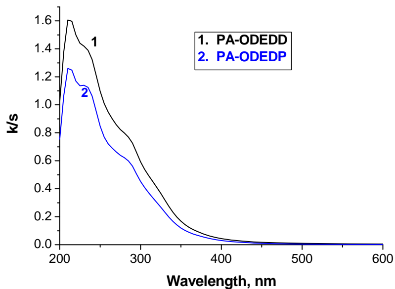
Fig. 13. UV-Vis spectra of PA-OEDDD and PA-OEDDP pulps, converted into k/s curves.
