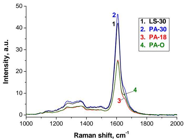
Fig. 4. UVRR spectra of low sulphidity pulp at kappa level 30 (LS-30), profiled alkali-cooked pulps at kappa levels 30 and 18 (PA-30 and PA-18, respectively), and profiled alkali-cooked pulp after oxygen delignification at kappa level 18 (PA-O).
