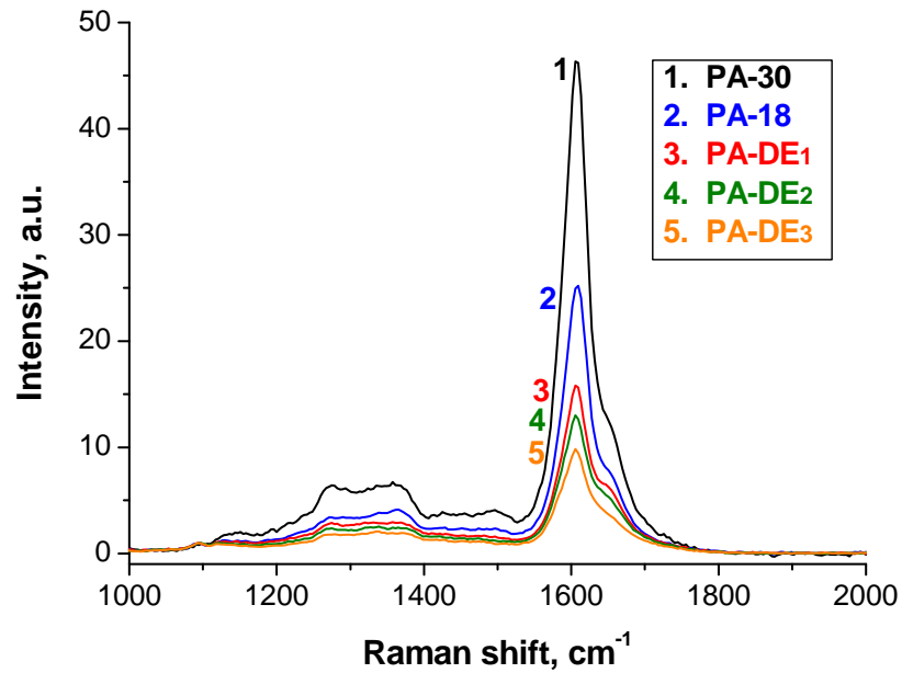
Fig. 6. UVRR spectra of profiled alkaline-cooked (PA) pulps at two different kappa levels (kappa 30 and 18) before and after chlorine dioxide bleaching. Chlorine dioxide charge increased in order PA-DE_1 < PA-DE_2 < PA-DE_3 .
