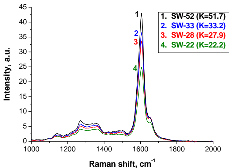
Fig. 2. UVRR spectra of unbleached softwood (SW) kraft pulps with kappa numbers 22-52. The heights of the spectra were normalized to the COC stretching band at 1098 \text{cm}^{-1} .
