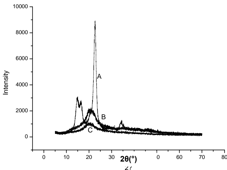
Fig. 5. XRD patterns of microcrystalline cellulose (A); treated by conventional heating (B); and cellulose treated by microwave(C)
