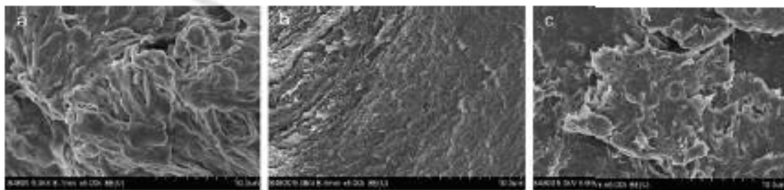
Fig. 4. SEM of microcrystalline cellulose (a); treated by conventional heating (b); treated by microwave (c)
