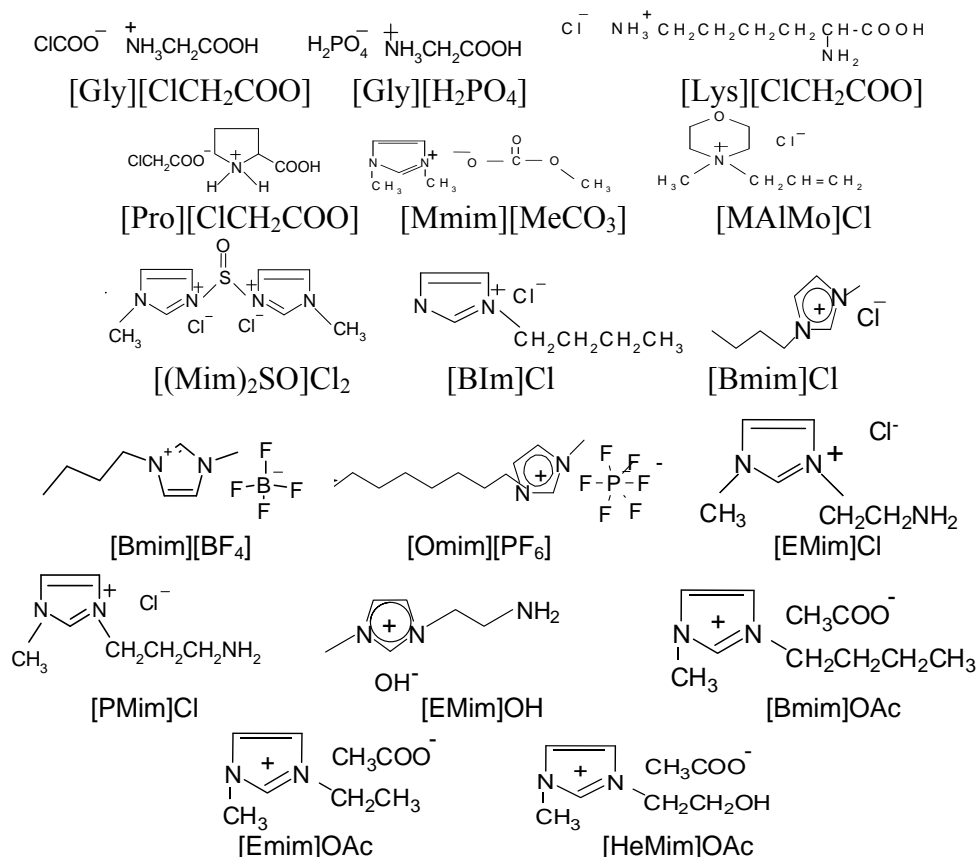
Fig. 1. Ionic liquids (ILs) prepared for use in the present study
