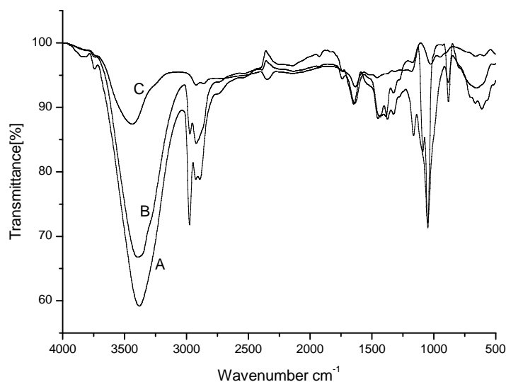
Fig. 3. FT-IR spectra of microcrystalline cellulose (A); treated with conventional heating (B); cellulose treated with microwave (C)
