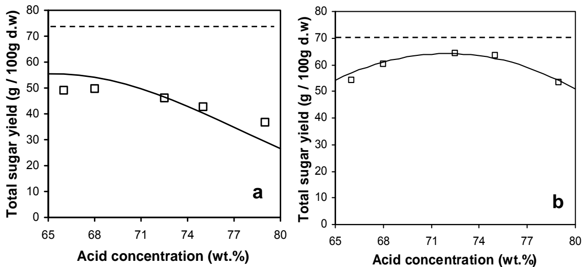
Fig. 4. Validation of the total sugar yields dependency on acid concentration at 35°C and 60 minutes. Experimental ( \square ) versus predicted (—), Theoretical maximum (----) (a) aspen (b) pine
