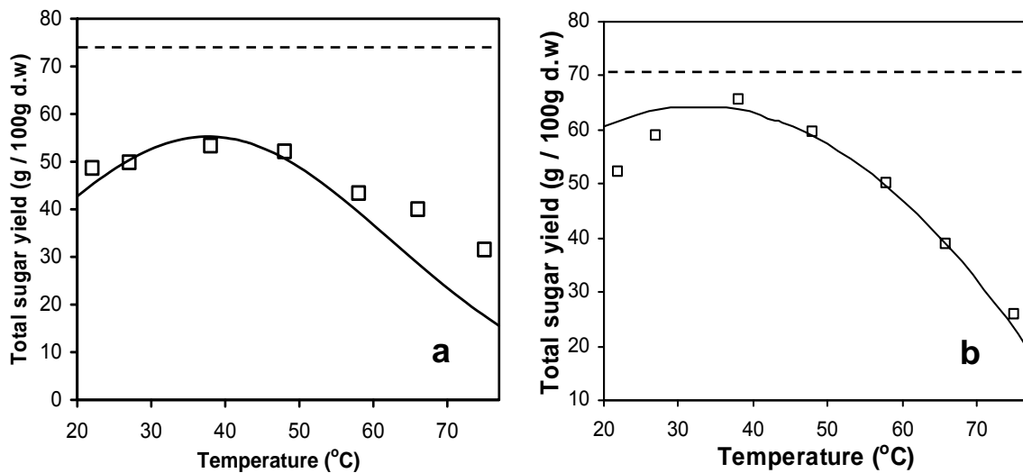
Fig. 5. Validation of total sugar yields dependency on temperature. Experimental ( \square ) vs predicted (—), Theoretical maximum (----) (a) aspen, 67 wt.%, 60 minutes (b) pine, 72 wt.%, 60 minutes
