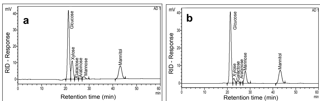
Fig. 1. Typical HPLC chromatogram profile for hydrolyzate obtained from a two-stage concentrated sulfuric acid process and separated on Chrompack Carbohydrates Pb column. Mannitol used as an internal standard. (a) aspen, (b) pine. Decrystallization conditions, measured monosugar concentrations and corresponding yields for these hydrolyzates are shown in Table 4.
