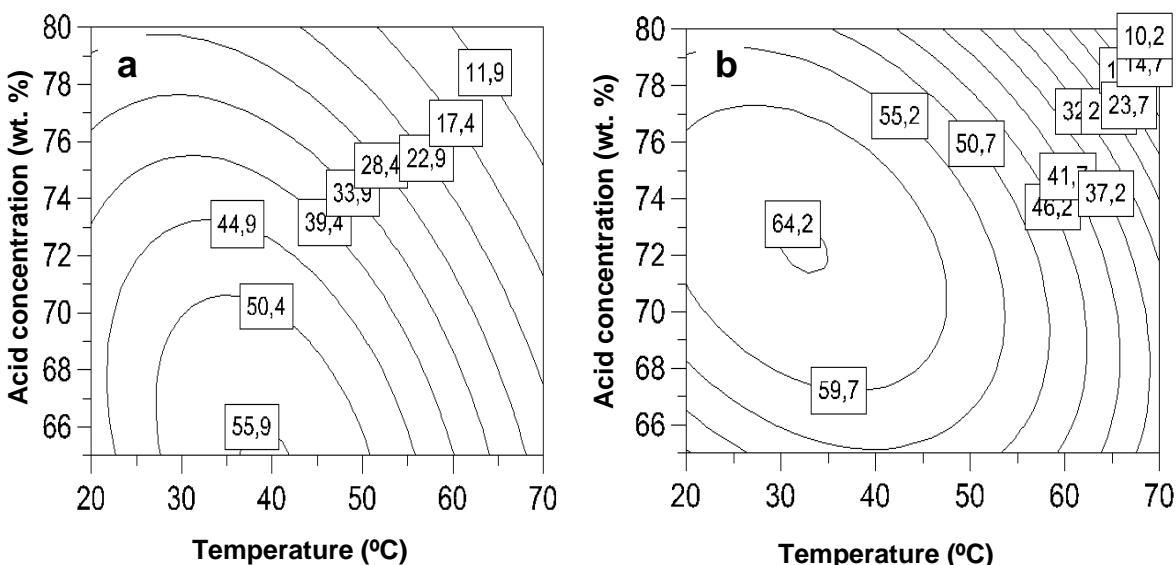
Fig. 3. Constant yield contour plots showing the effect of temperature and acid concentration on the total sugar yield at decrystallization time of 60 minutes (a) aspen (b) pine
