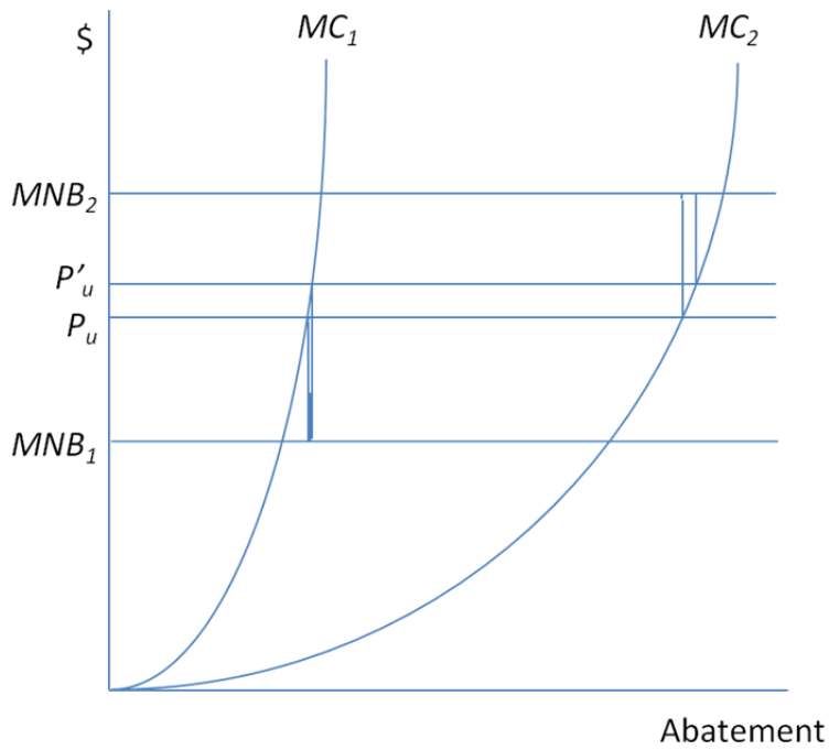
Figure 1B. Efficiency loss with uniform pollution price: Heterogeneity in marginal benefits and marginal costs.
