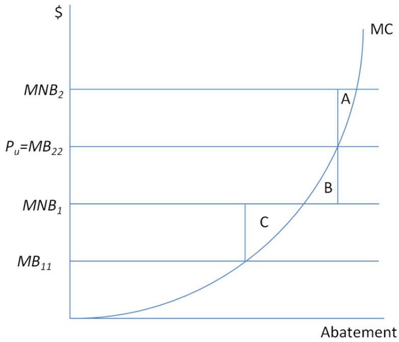
Figure 1B. Efficiency loss with uniform pollution price: Heterogeneity in marginal benefits and marginal costs.
