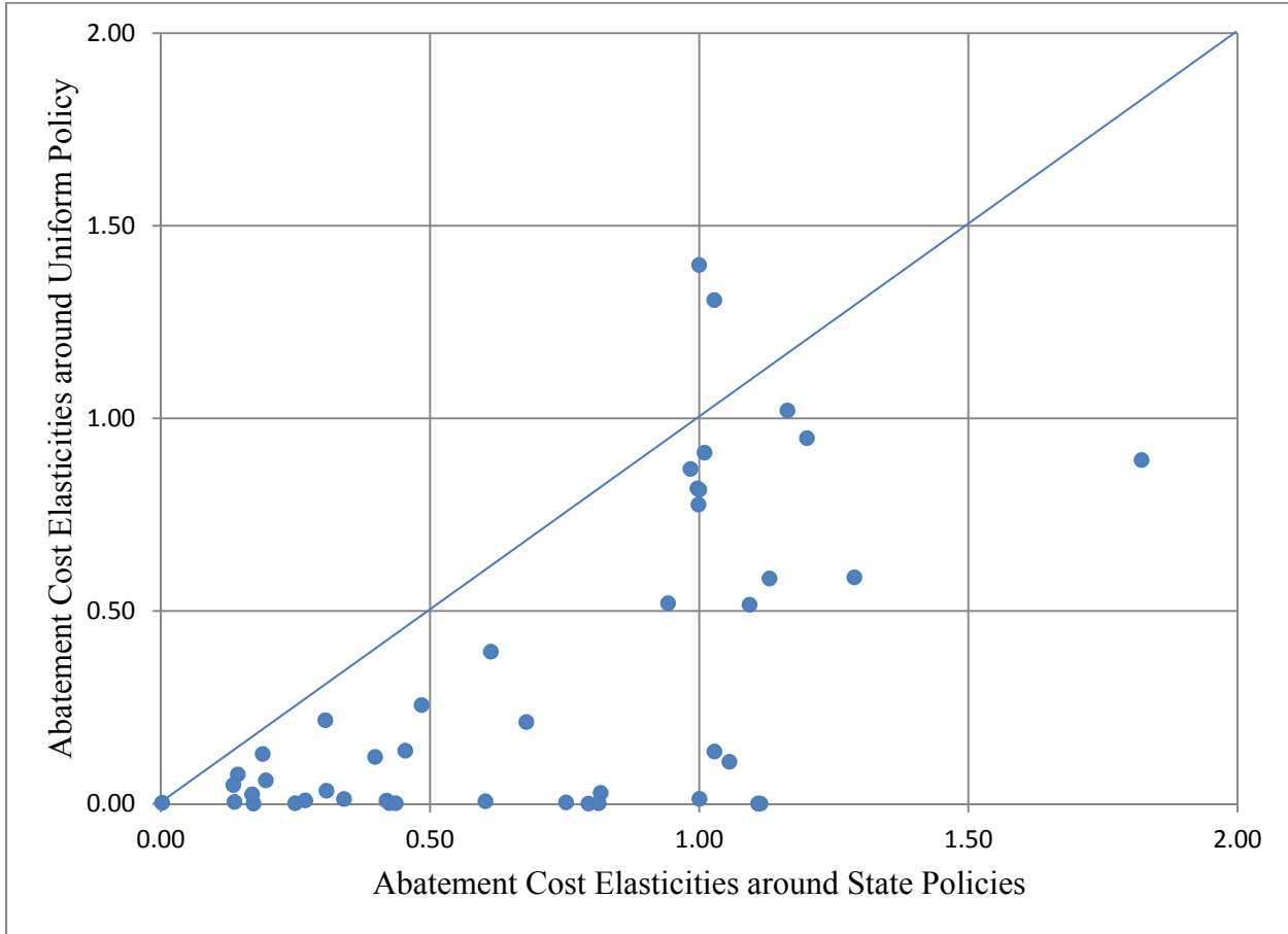
Figure 6. Elasticities of Marginal Abatement Costs around Equilibria for State and Uniform Policies
