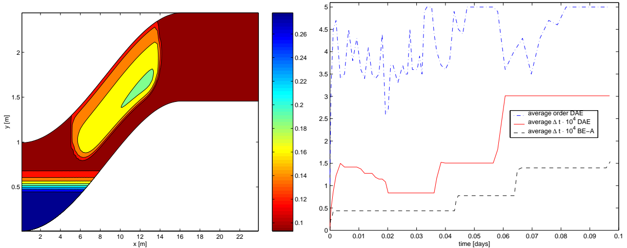
Figure 1. left: Spatial distribution of water phase volume fraction for hill-slope simulation. right: Temporal integration order and step size as a function of simulation time for hill-slope simulation.
