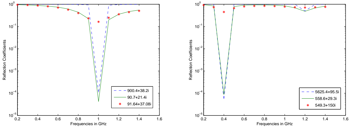
Figure 2: Reflection coefficients calculated using (\epsilon_{jR}, \mu_{jR}) from materials 1R, 2R, and 3R which are associated with (900.4+38.2i, 1), (90.7+21.4i, 10+2i) , and (91.64+37.08i, 10+2i) , respectively (left) and materials 4R, 5R, and 6R which are associated with (5625.4+95.5i, 1), (558.6+29.3i, 10+1.2i) , and (549.3+150i, 10+2i) , respectively (right).
