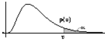
Figure 1: Example of U \sim \chi^2(4) density
