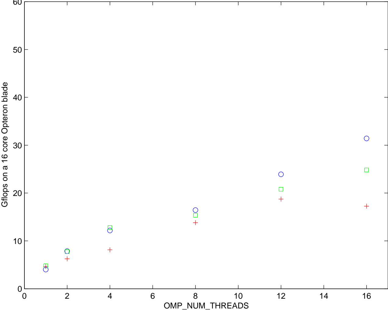
Gflop rates for Long Tall BLAS-3 --- 380K by 40 --- gfortran with ACML library
