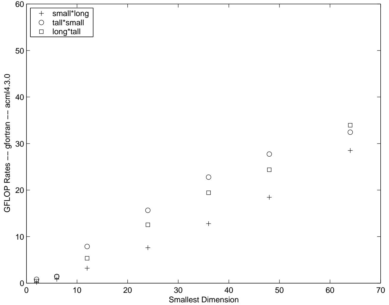
16 Core GFLOP Rates for Long Skinny BLAS -- gfortran -- acml4.3.0
