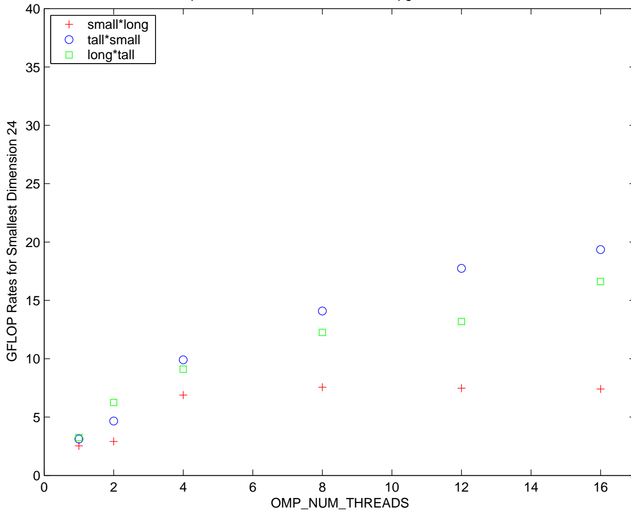
Gflop Rates vs. Number of Threads --- pgf90 --- acmlBLAS
