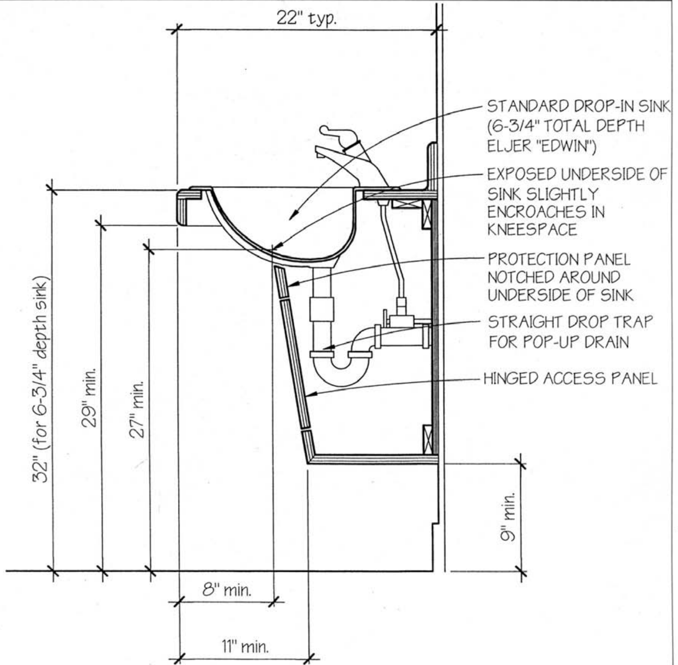
SECTION OF LAVATORY WITH PIPE PROTECTION PANEL, 32" COUNTER HEIGHT In this scheme, the counter height is the standard 32" height. The bottom of the sink encroaches slightly into the standard knee space, and the protection panel must be notched around the underside of sink.
