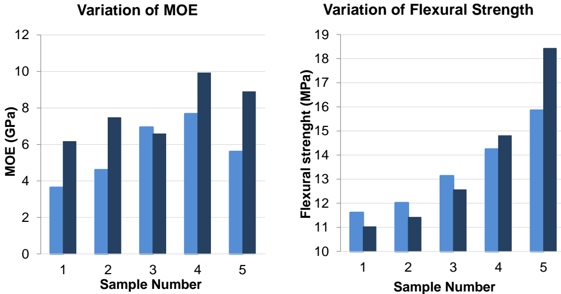
Fig. 5. MOE and flexural strength values for composites (reference samples 1 to 5) cured at 28 days (light color) compared with aged ones (dark color)
