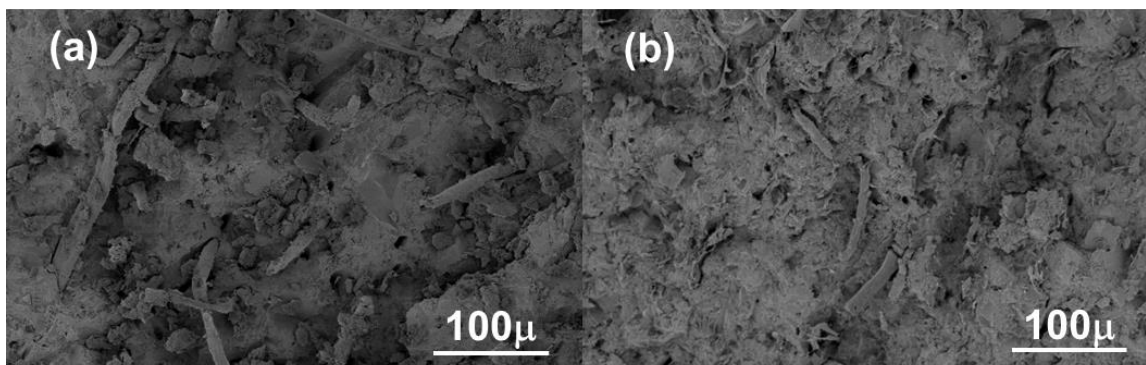
Fig. 3. SEM of the fracture surface of composite reinforced with 8 wt% (250x) of (a) conventional pulp (reference sample 1) and (b) nanofibrillated pulp (reference sample 5)
