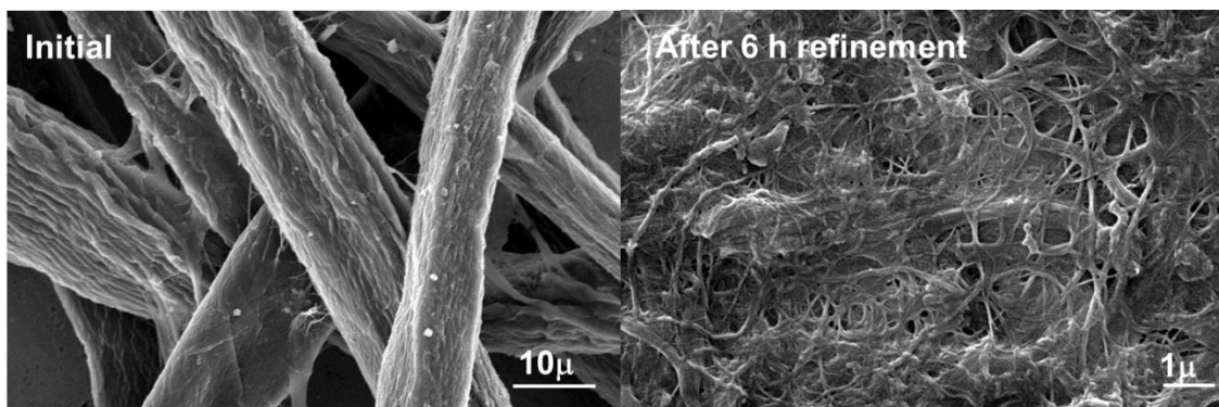
Fig. 1. SEM micrographs of the initial sisal pulp (2,000x) and sisal pulp after 6 h refinement (10,000x)
