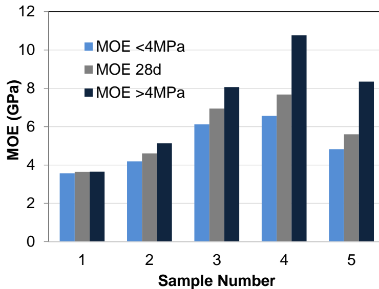
Fig. 4. MOE values calculated for the reference samples 1 to 5 for strengths higher than 4 MPa and lower than MPa, compared with average MOE values
