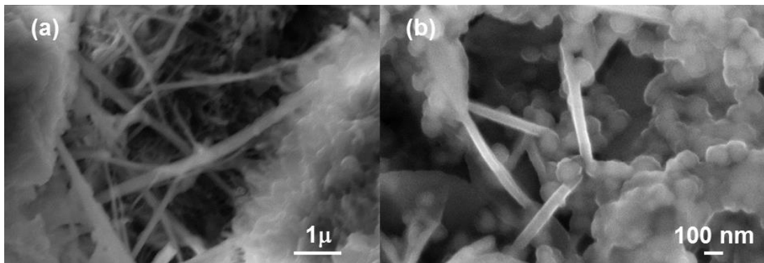
Fig. 6. BSEM of the fracture surface of composite reinforced with 8 wt% of nanofibrillated pulp (a) detail of nanofibrillated cellulose intermixed with cement matrix particles –unaged composite– (40,230x) and (b) detail of the dispersion of fibers on the matrix (141,890x) –aged composite–
