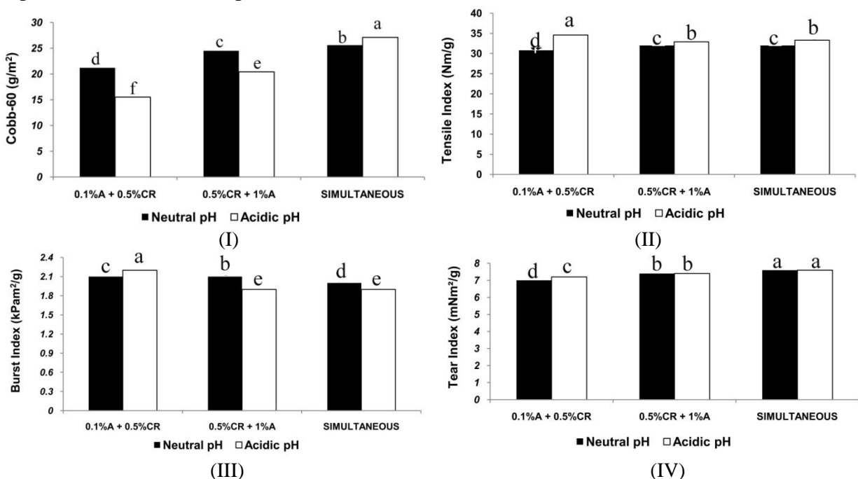
Fig. 5. Effect of pH and alum/cationic rosin sequence of addition on water resistance (I) and mechanical properties (II, III, and IV) (A: Alum and CR: Cationic Rosin)
