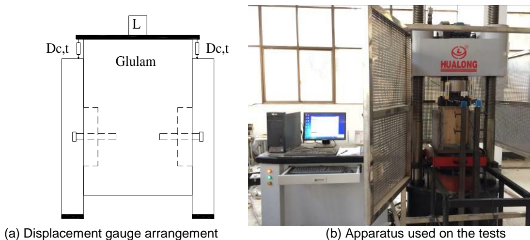
Fig. 5. Apparatus used on the tests
