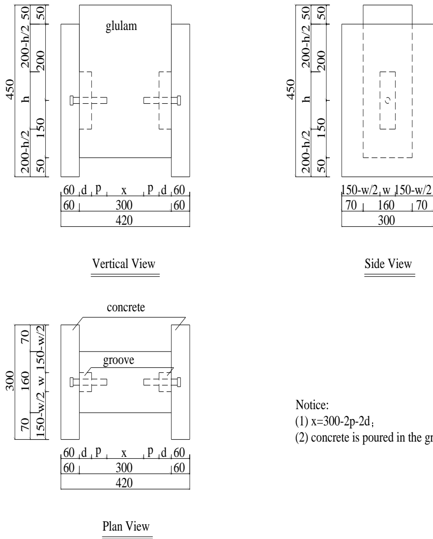
Fig. 4. Drawing of timber-concrete composite push-out samples (Unit:mm)
