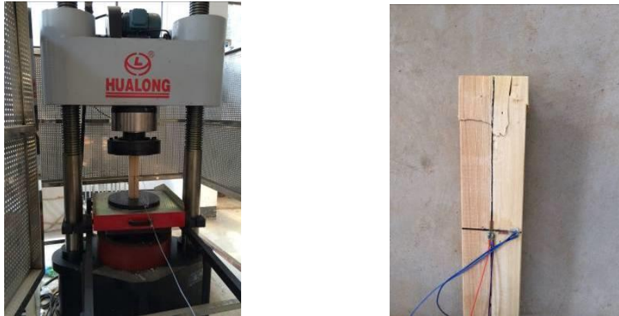
Fig. 2. Compressive strength tests of timber
