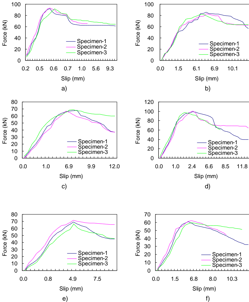
Fig. 6. Load-slip curves for all test groups: a) T-1; b) T-2; c) T-3; d) T-4; e) T-5; and f) T-6
