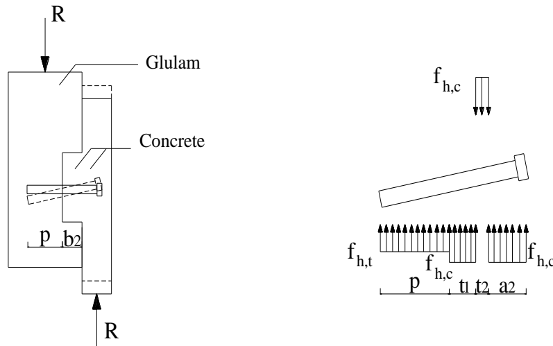
Fig. 1. Mechanism of stud-groove-type connectors failure: a) failure mode with two plastic hinges, one hinge in concrete and another in glulam; b) failure mode with two plastic hinges, both hinges in concrete; c) failure mode with one plastic hinge, with the intersection of stud before and after failure in glulam; d) failure mode with one plastic hinge, with the intersection of stud before and after failure in concrete in the groove; e) failure mode with rotation, with the intersection of stud before and after failure in glulam; and f) failure mode with rotation, with the intersection of stud before and after failure in concrete in the groove
